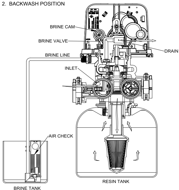
2. BACKWASH POSITION
